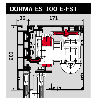
8 Enhanced operator with sound-insulated motor mounting, low-noise, replaceable track rail and increased motor capacity
