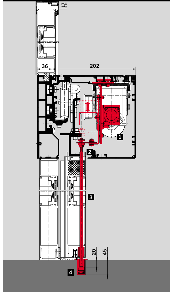
ST-R/ES with concealed-rod locking system
