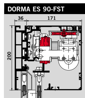
5 Standard operator with low-noise track rail
