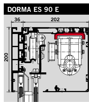
2 Standard operator with low-noise track rail, sound-insulated motor mounting and increased motor capacity
