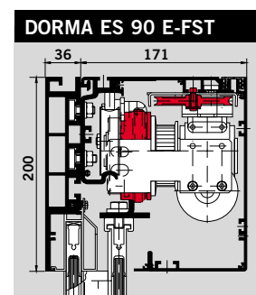
6 Standard operator with low-noise track rail, sound-insulated motor mounting and increased motor capacity
