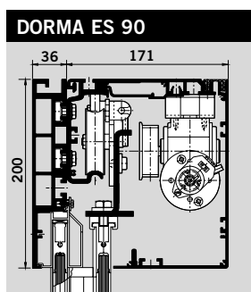
1 Standard operator with low-noise track rail
